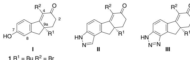
Figure 1. ER \beta ligands based on tetrahydrofluorenones.
